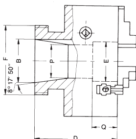
DIN 55026 Mounting from front Available on request!
