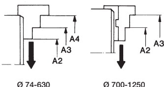
Internal chucking
