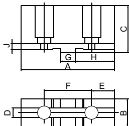
Reversible top jaw UB
