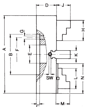
Cylindrical centre mount
