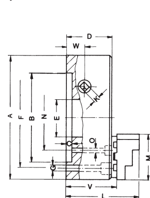
Cylindrical centre mount
