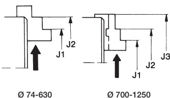
Internal chucking
